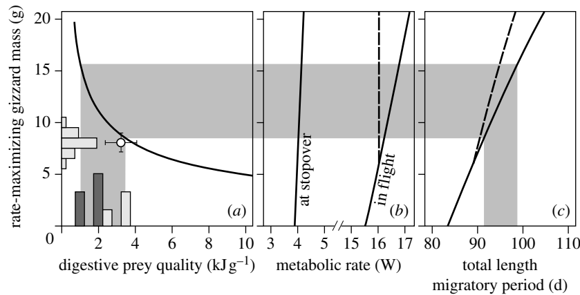
Figure 5. The predicted effect of digestive prey quality at stopovers on overall speed for a theoretical, but realistic, knot population to migrate 15 000 km from wintering to breeding grounds. (a) Expected net-rate maximizing gizzard mass declines with prey quality (solid curved line; see eq. given in §2). Given the observed frequency distribution of prey qualities among sites (bars on horizontal axis), knots only select stopovers that harbour the highest prey qualities (light grey bars; dark grey bars represent wintering sites). As predicted, gizzards observed at stopovers are distributed around 8 g (bars on vertical axis). Mean stopover gizzard mass versus mean stopover prey quality is given by open dot (bars are 95% confidence intervals). (b) Metabolic rates are predicted to increase as a function of gizzard size, especially during flight. (c) Through these higher energetic costs, the total length of the migratory period increases with increasing gizzard size (i.e. declines with increasing prey quality). Grey band across the three figures shows that, according to the model, stopping over in the best instead of in the worst sites should reduce length of migratory period by about a week. Downsizing the gizzard before flight (to 6 g with no time or energy costs of transformation), results in only a minor reduction of the migratory period (dashed line in b and c ).
